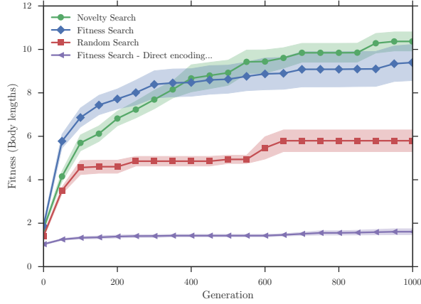
Figure 7: Simple genetic algorithm against novelty-fitness-random search with generative encoding. Best fitness so far averaged over 10 runs.
