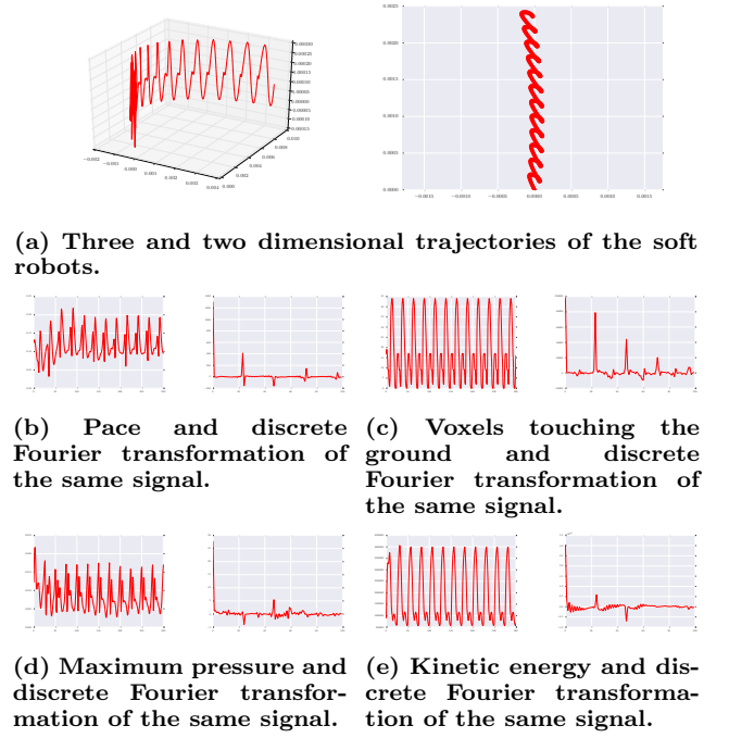
Figure 4: Observed behaviors of the soft robots used for the sparsity computation in novelty search.
